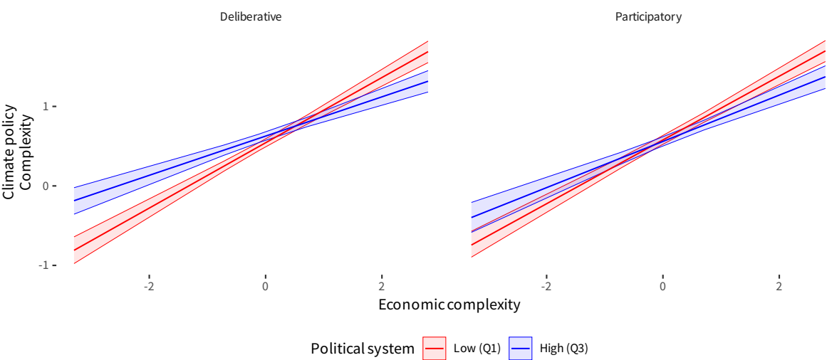
Figure S0.2: Effects. Shannon diversity.
