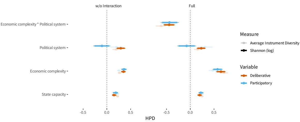
Figure S0.1: Comparison with different measures of diversity.
